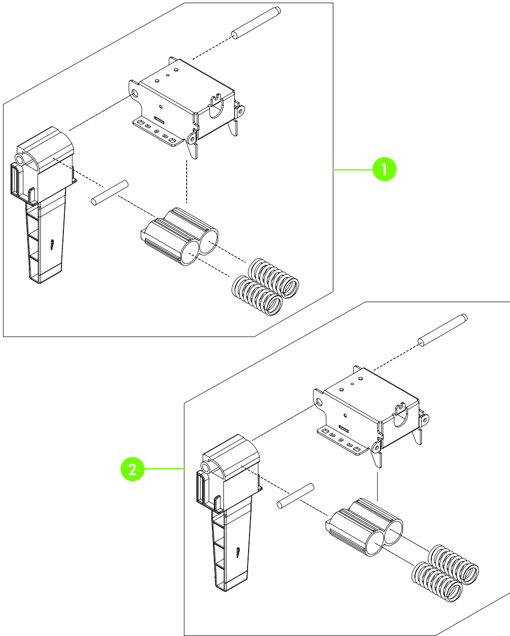
Figure 7-33 ADF internal components (2 of 3)
