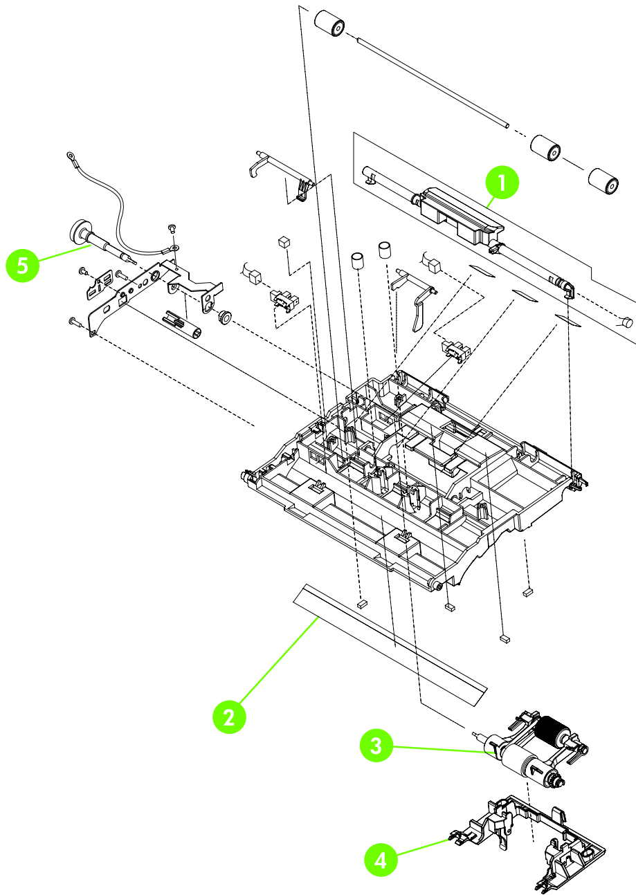
Figure 7-34 ADF internal components (3 of 3)
