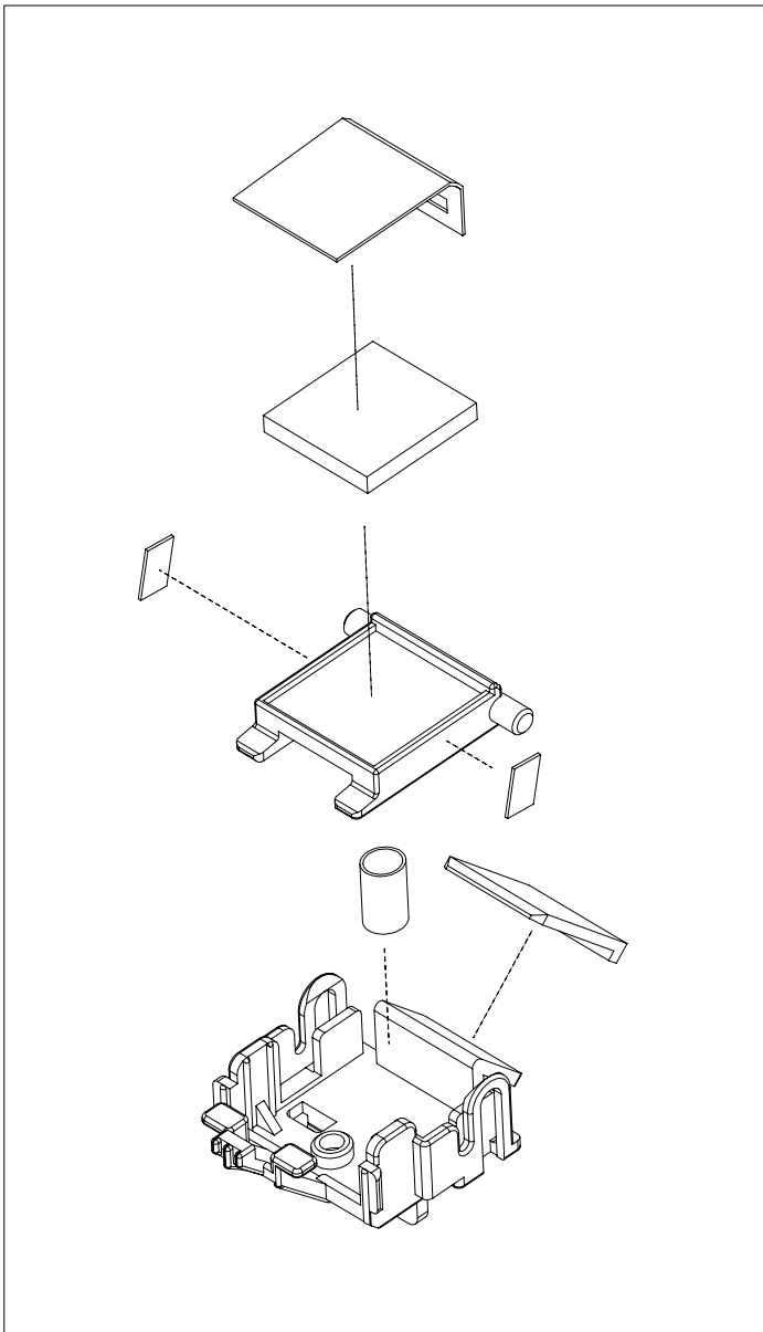
Figure 7-36 ADF separation pad
