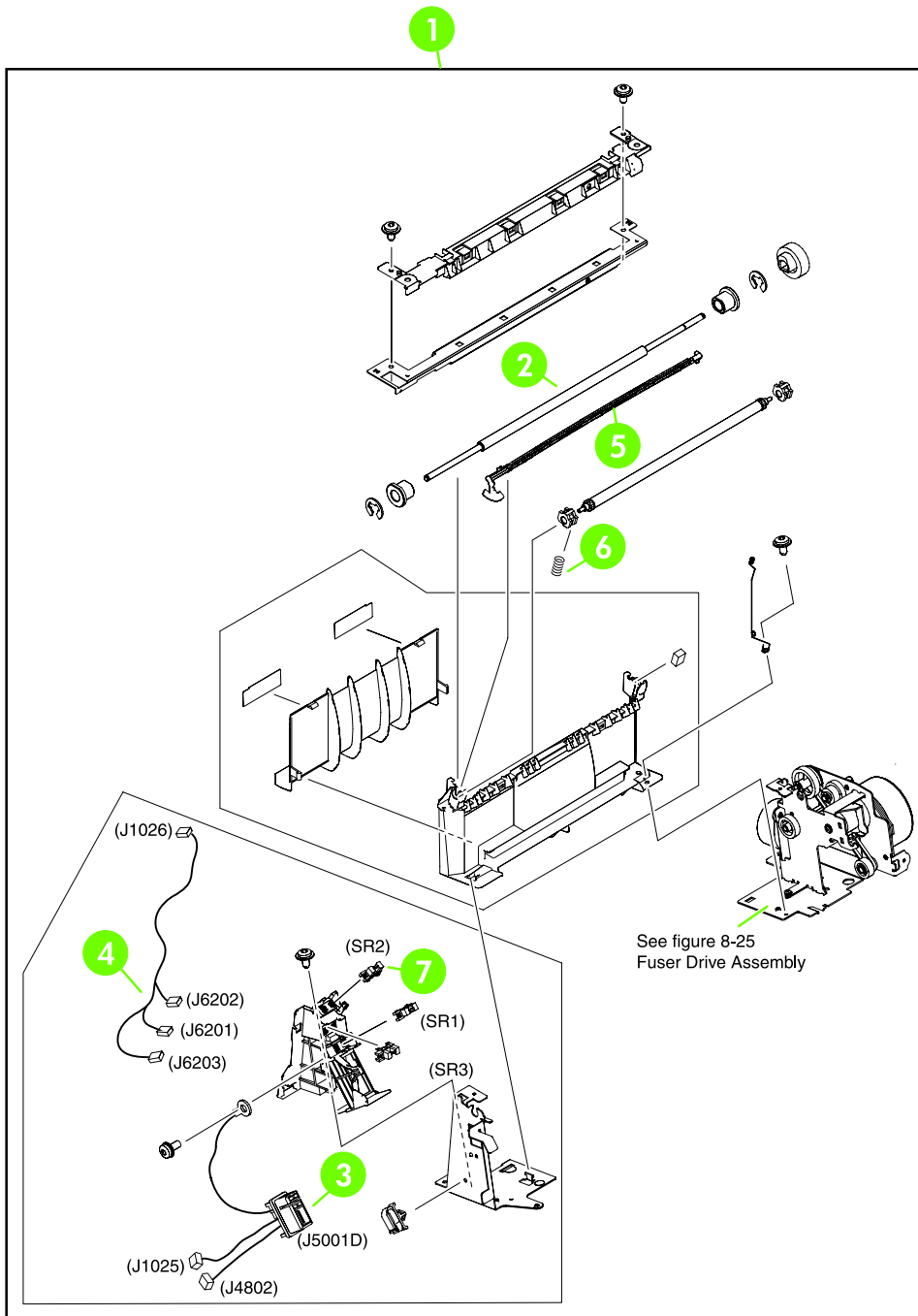
Figure 7-24 Delivery assembly
