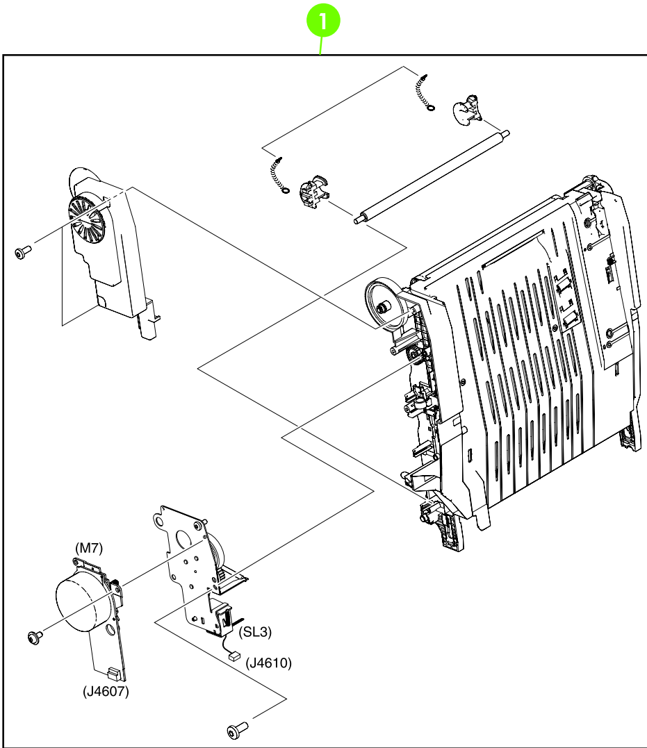
Figure 7-23 ETB assembly
