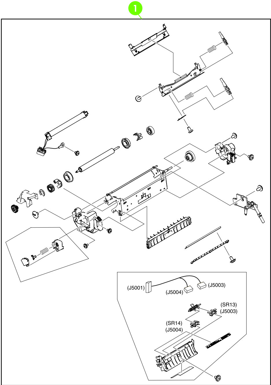
Figure 7-29 Fuser assembly
