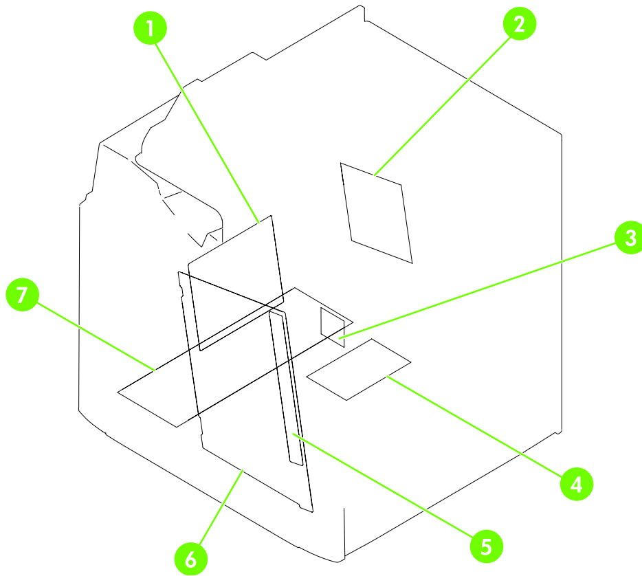
Figure 7-30 PCB assembly
