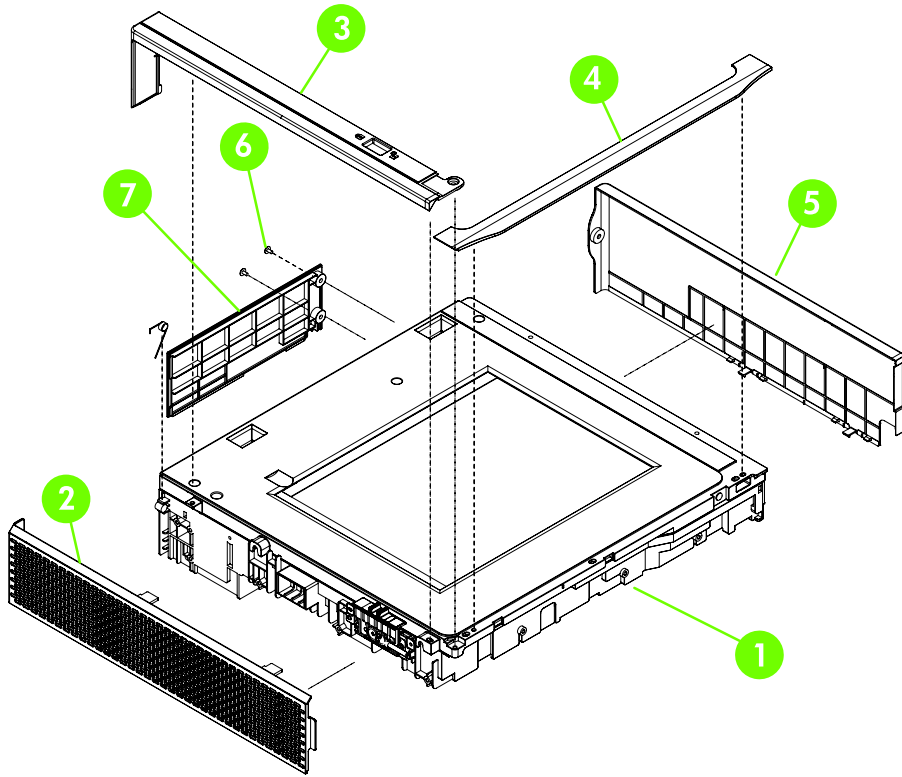
Figure 7-43 Scanner covers
