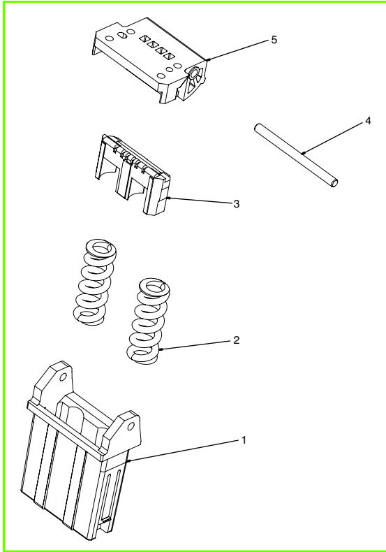
Figure 9-75 Hinge assembly
