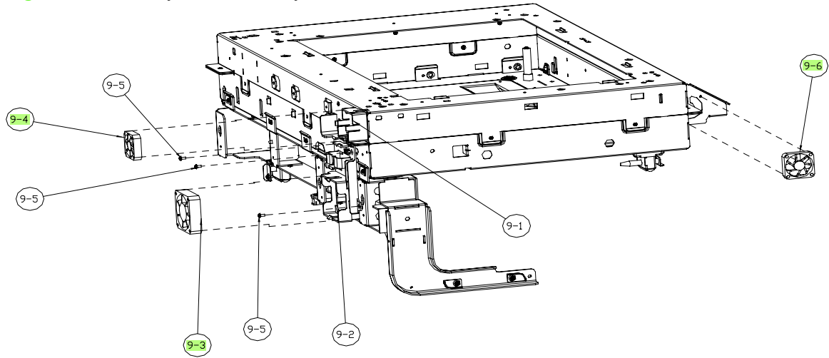
Figure 9-99 Fan-system assembly
