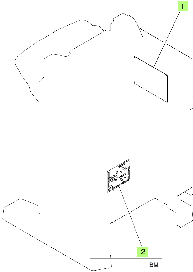
Figure 9-72 PCA assembly
