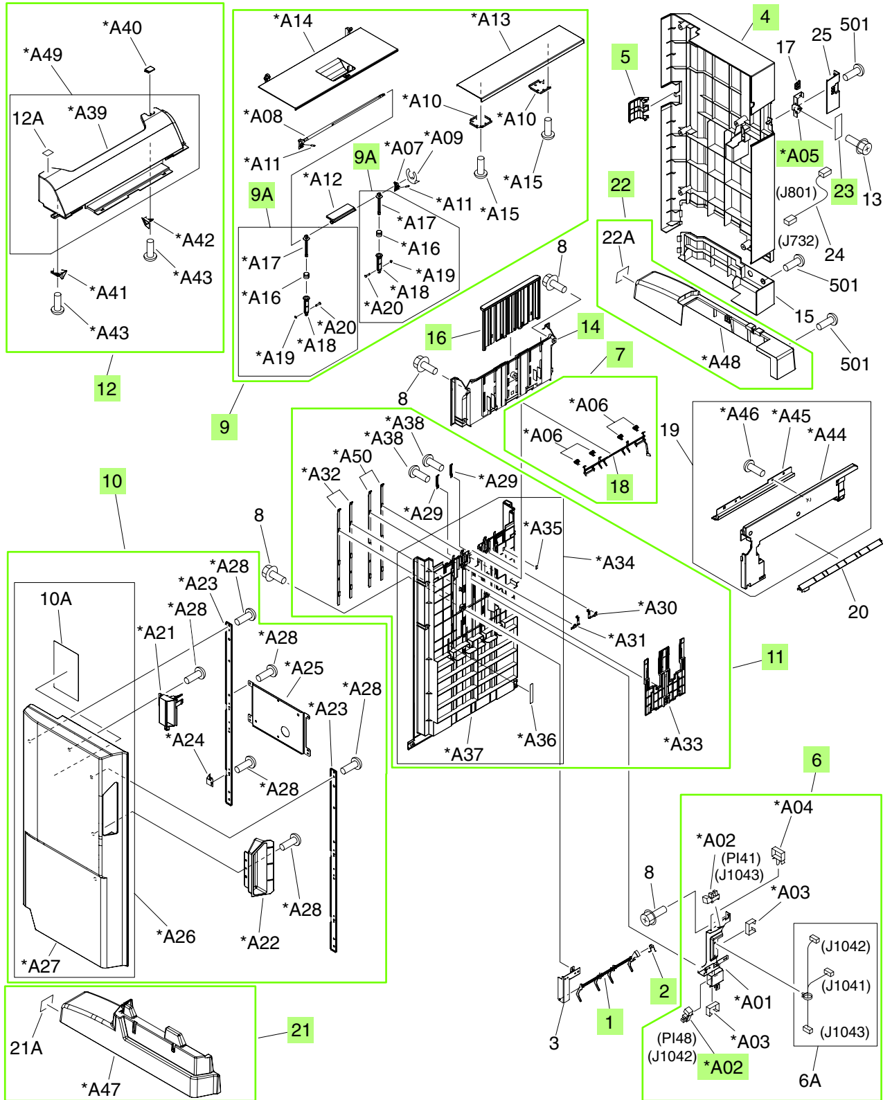
Figure 9-37 External panels and covers (stapler/stacker)
