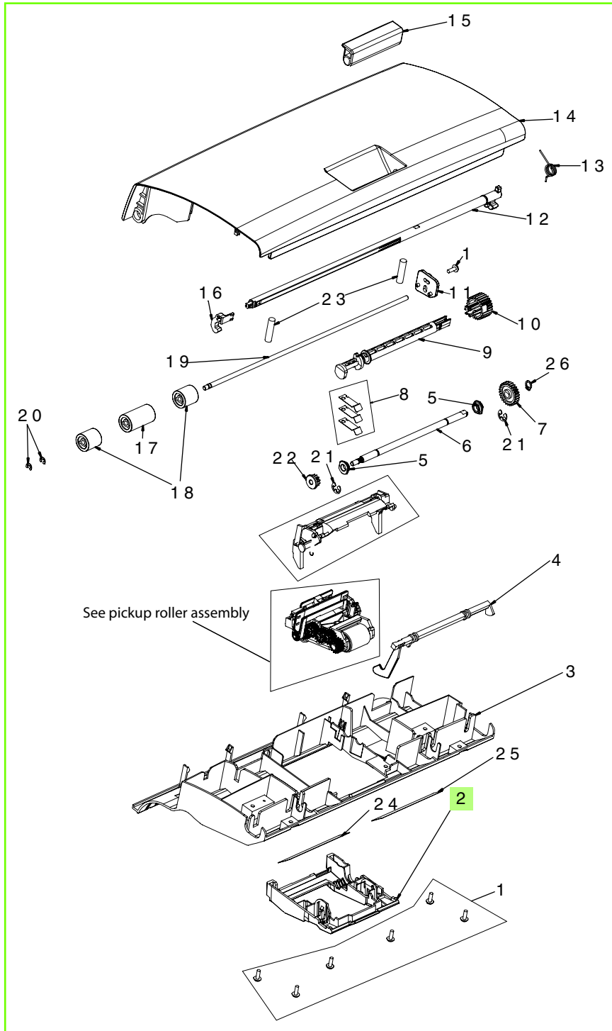
Figure 9-78 Jam-cover assembly
