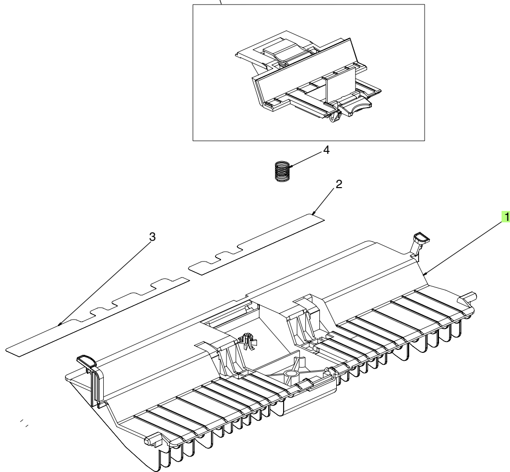
Figure 9-81 Separation-floor assembly See separation pad assembly
