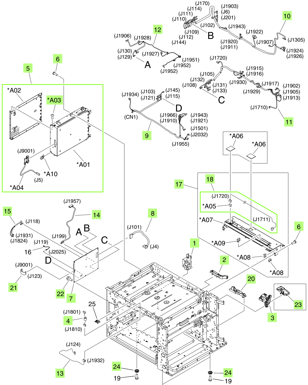
Figure 9-9 Printer internal components (6 of 7)
