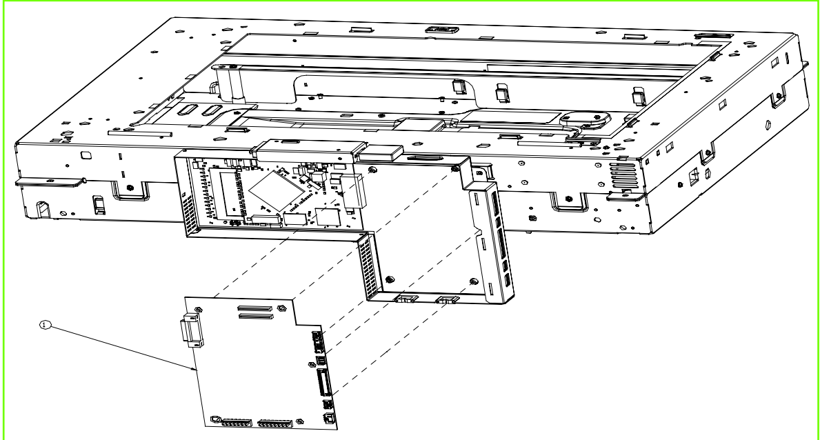
Figure 9-84 Scanner controller-board (SCB) assembly
