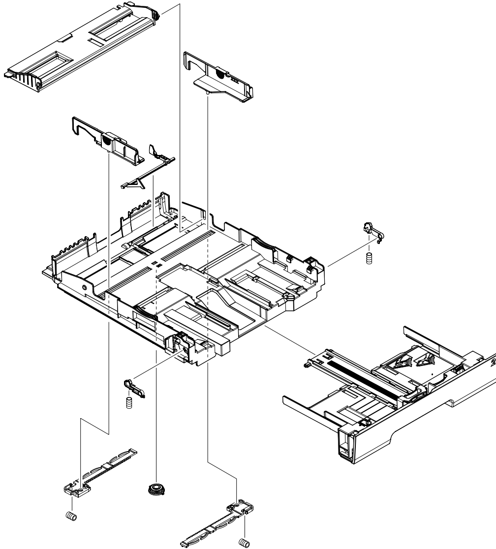
Figure 8-7 Cassette
