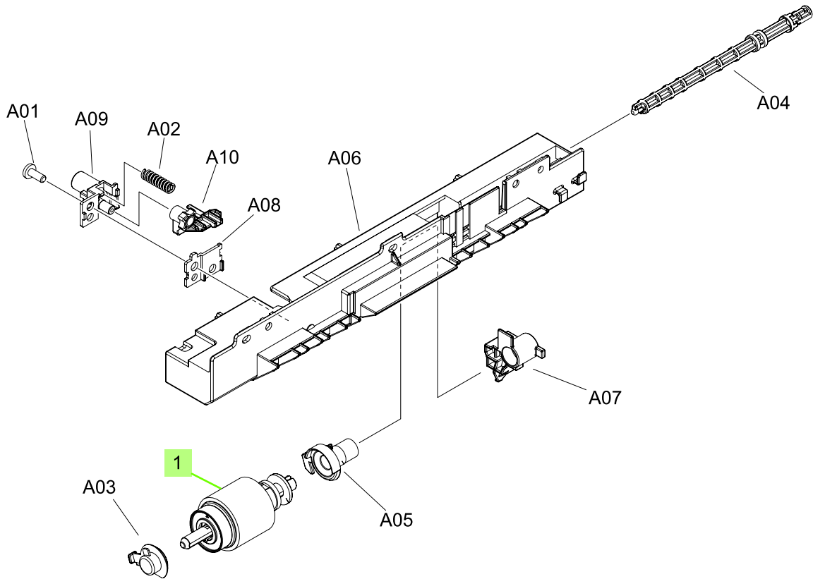
Figure 8-9 Cassette paper pickup assembly
