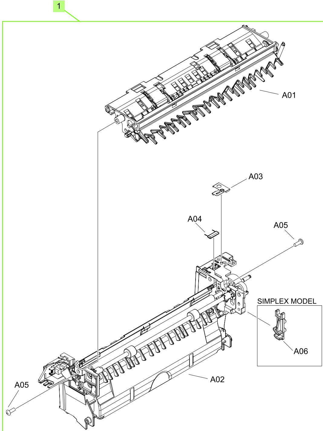
Figure 8-13 Delivery assembly
