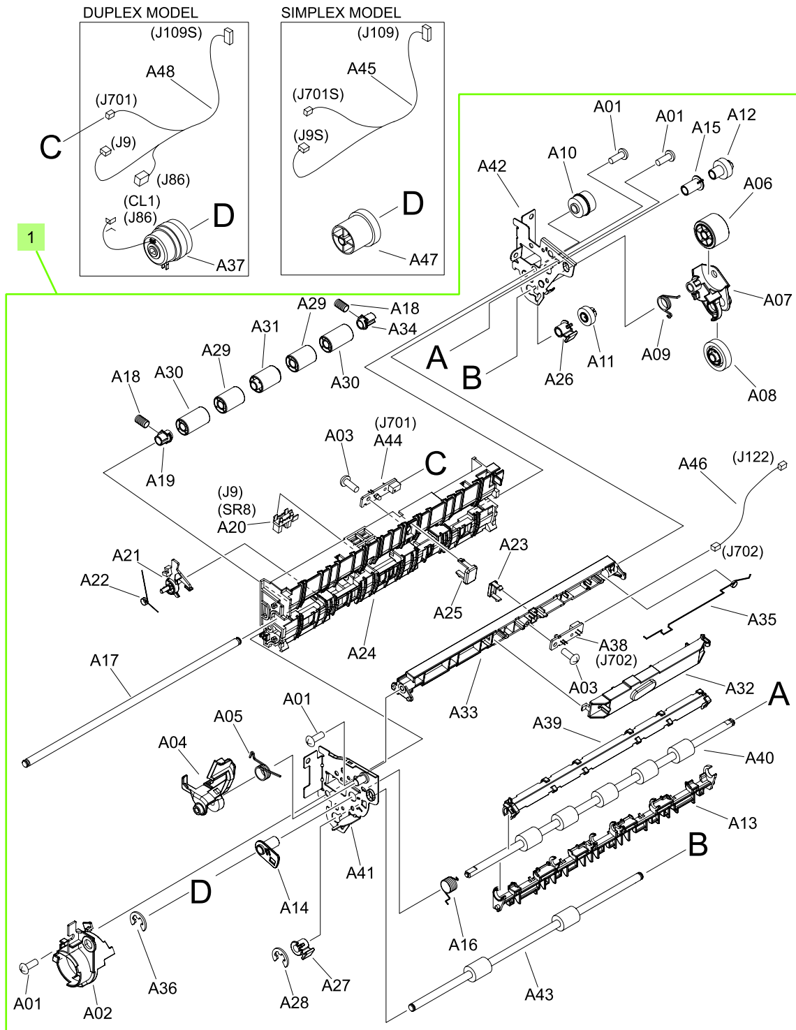
Figure 8-11 Registration assembly
