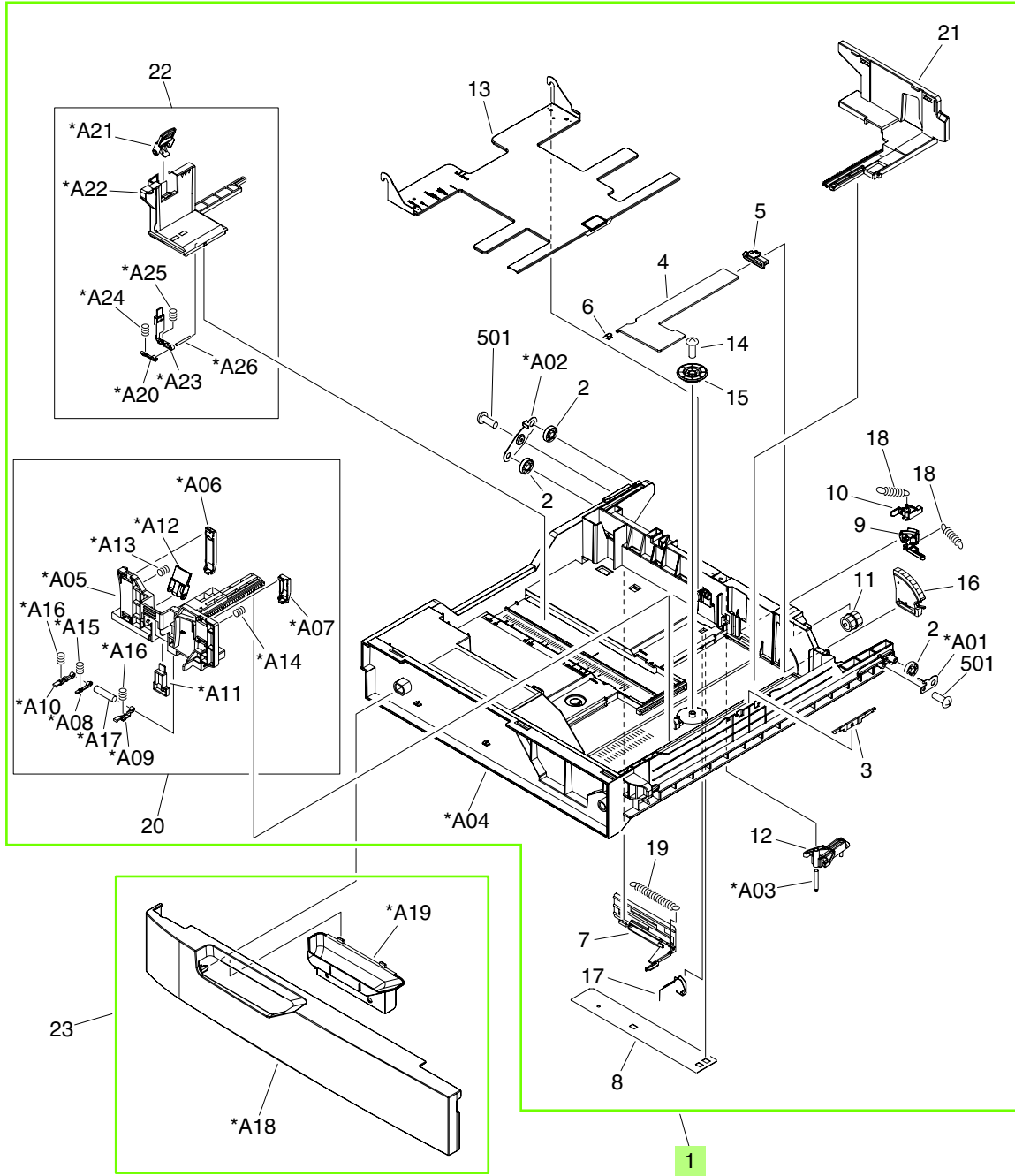
Figure 9-15 Printer cassette
