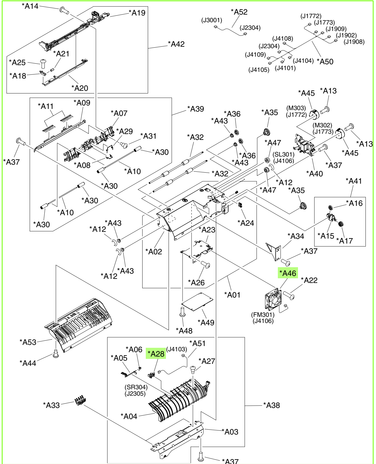
Figure 9-21 Printer duplexing-reverse assembly (duplex model)
