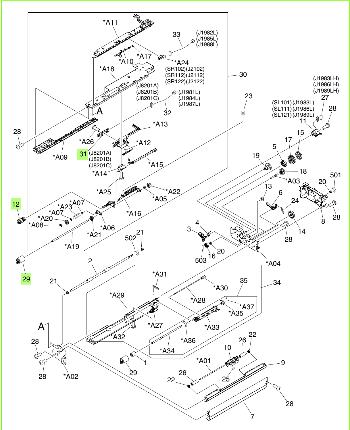
Figure 9-30 Input-tray paper-pickup assembly
