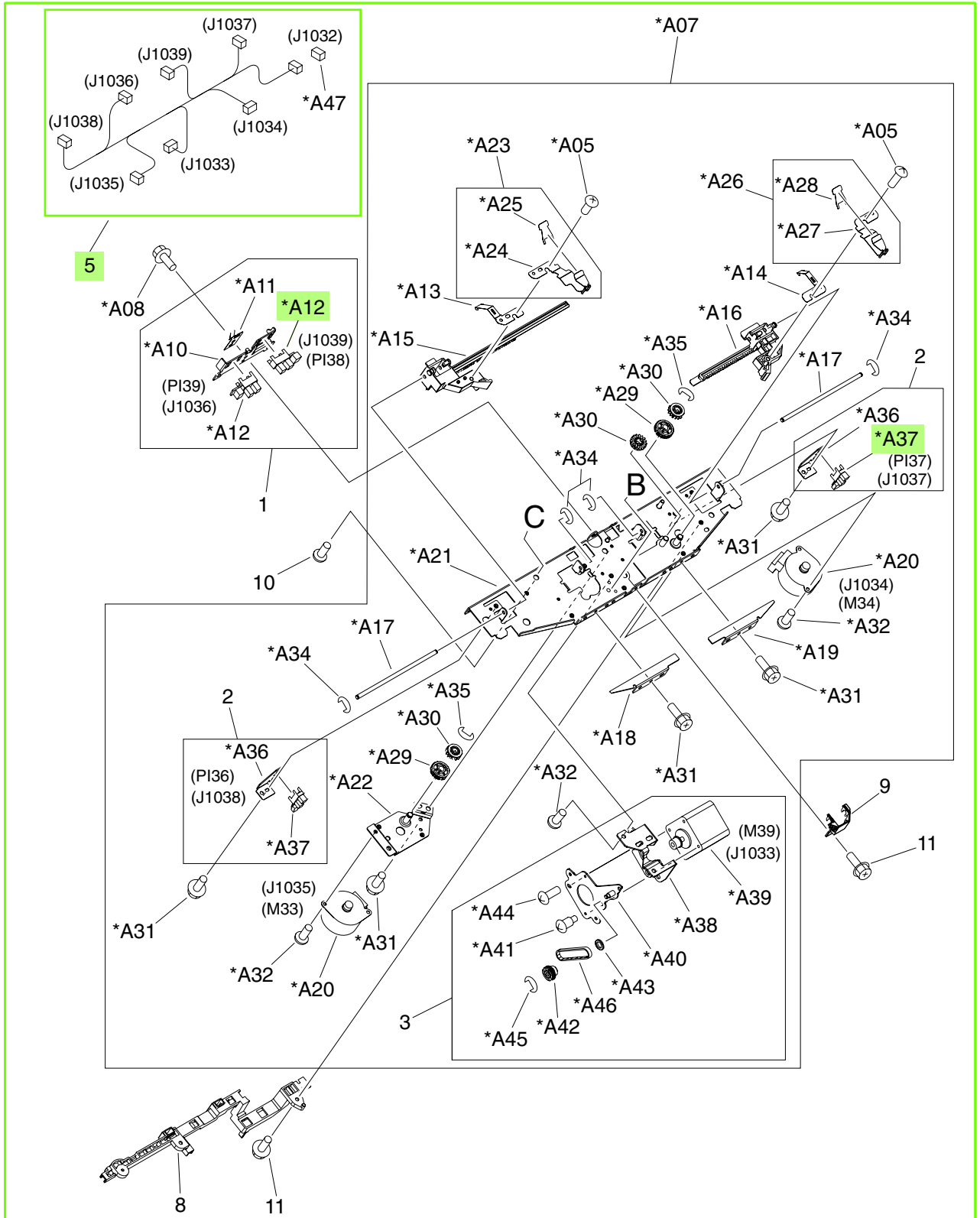
Figure 9-53 Operation-tray assembly (2 of 2) (stapler/stacker and booklet-maker)
