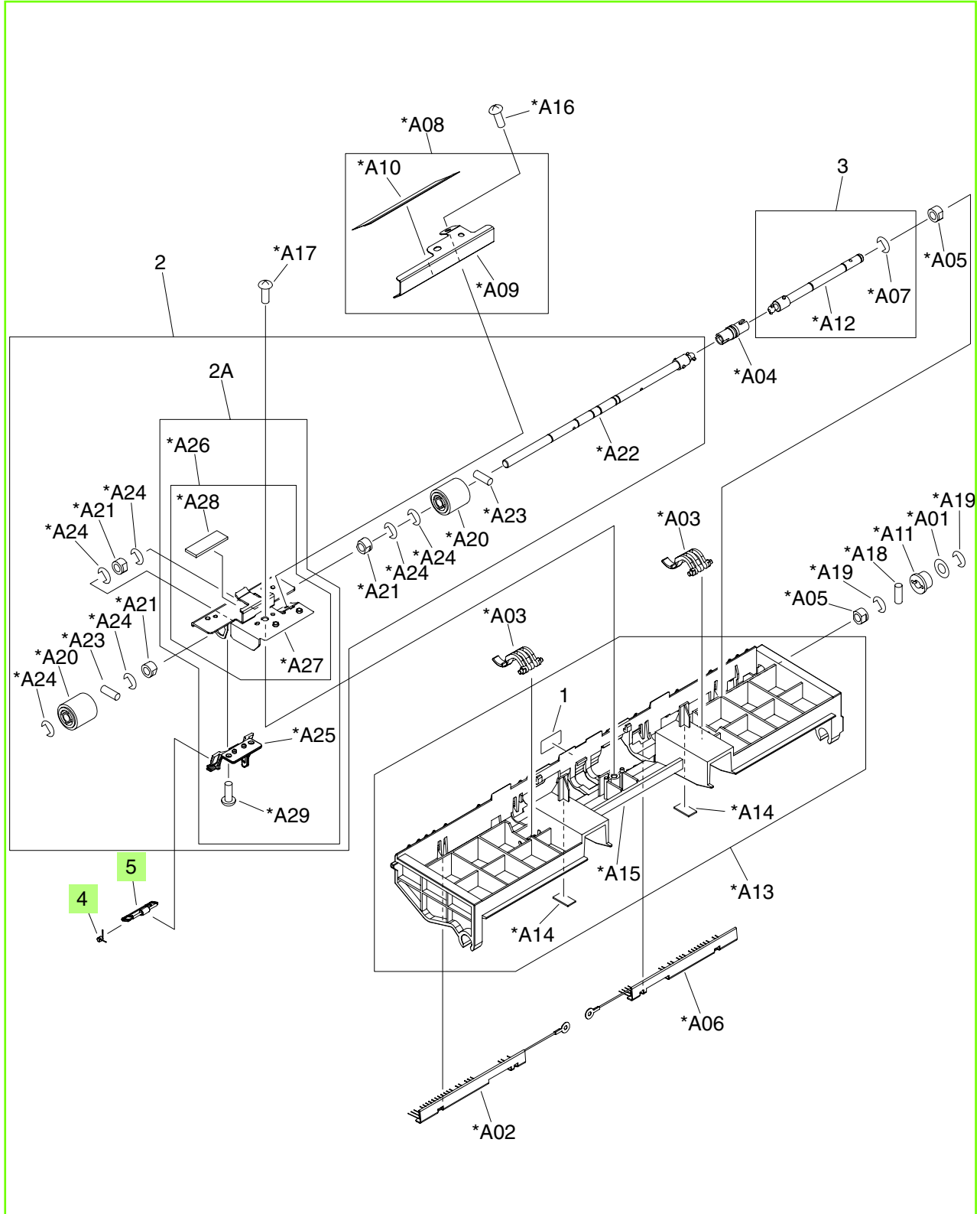
Figure 9-57 Swing-guide assembly (stapler/stacker and booklet-maker)
