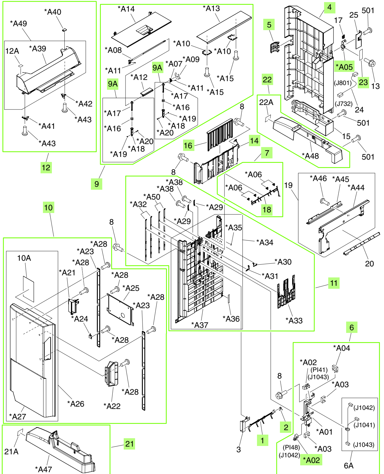
Figure 9-38 External panels and covers (stapler/stacker)
