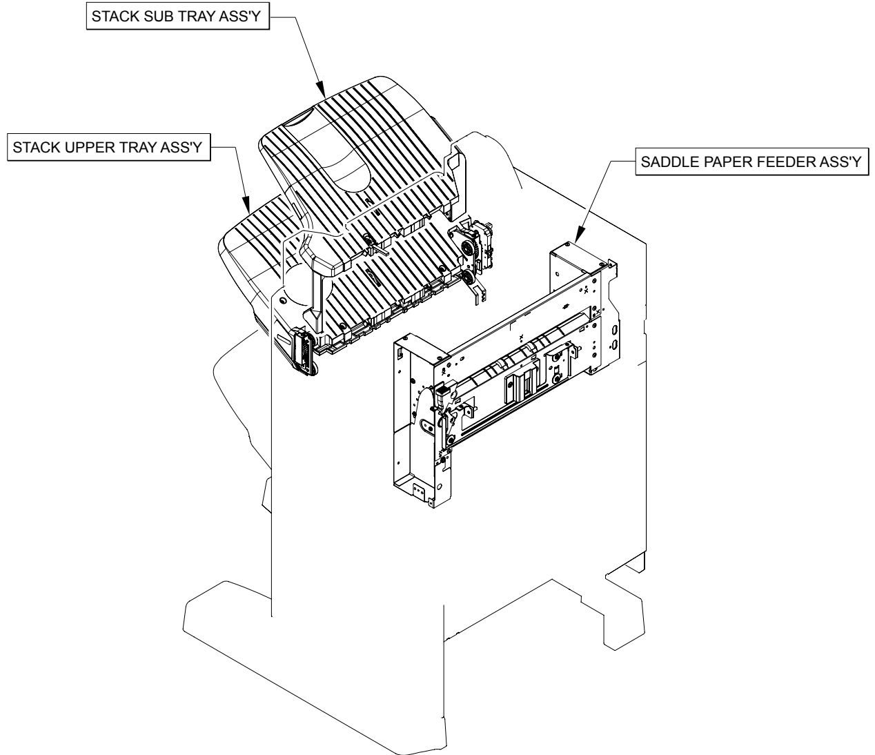
Figure 9-36 Stapler/stacker unit
