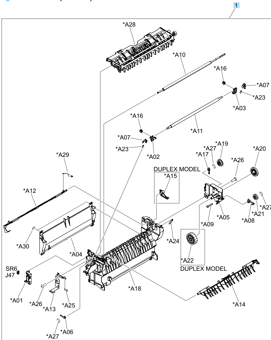
Figure 4-16 Delivery assembly
