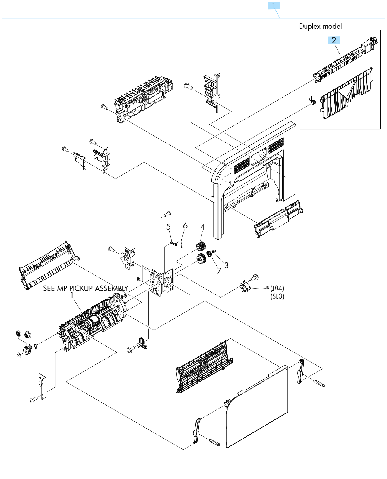
Figure 4-2 Right-door assembly
