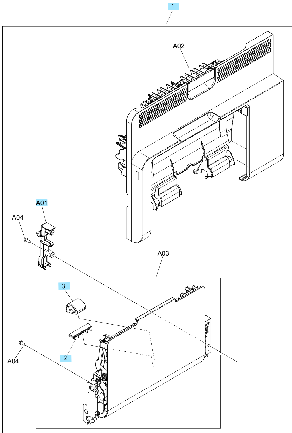
Figure 2-7 Right door
