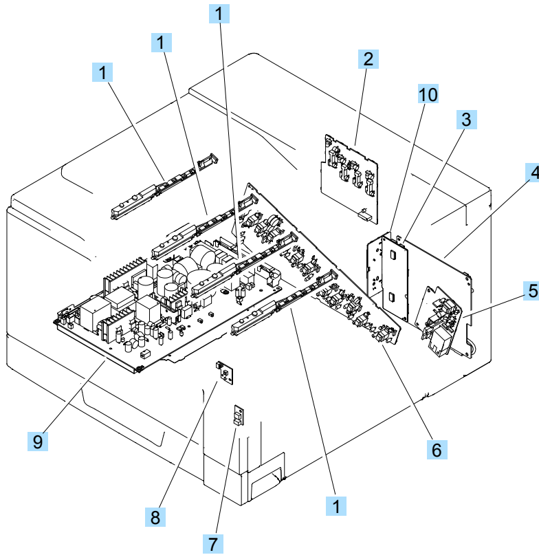
Figure 4-15 PCAs
