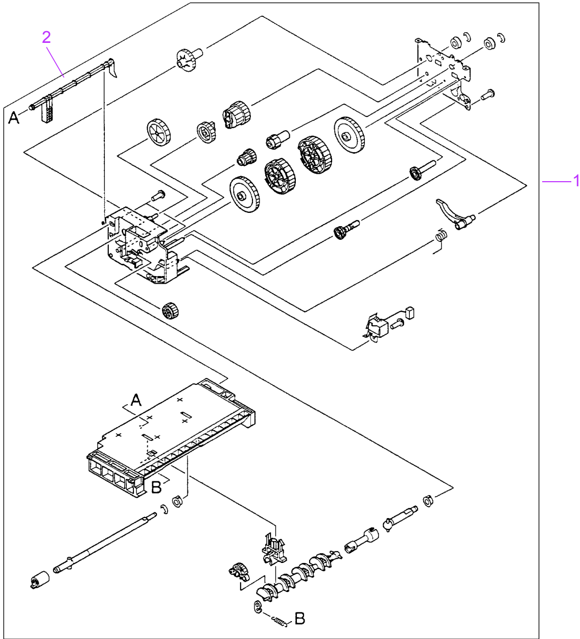
Figure 8-24 Lower Paper Pickup Drive Assembly
