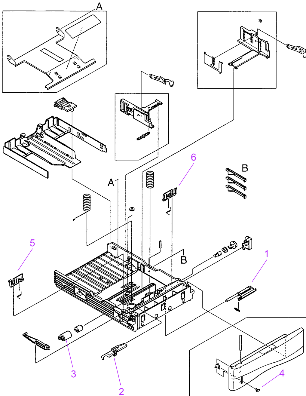
Figure 8-25 250-sheet Tray
