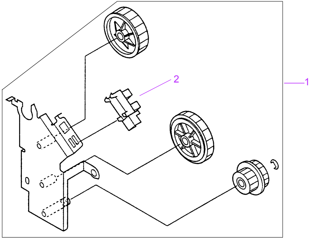
Figure 8-8 Delivery Drive Assembly
