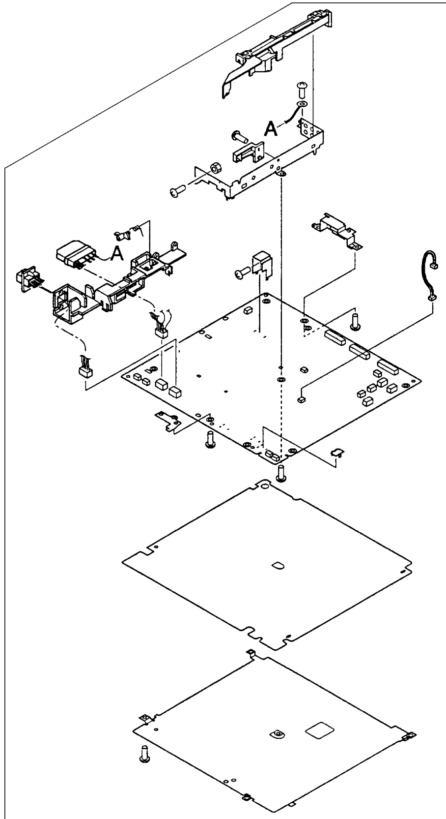
Figure 8-7 Engine Controller Board Assembly
