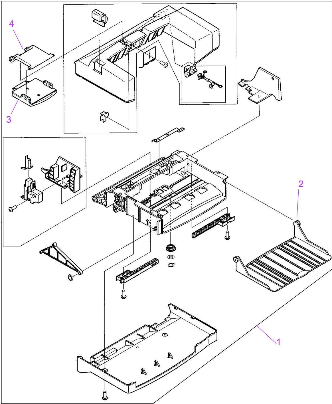
Figure 8-28 Envelope Feeder
