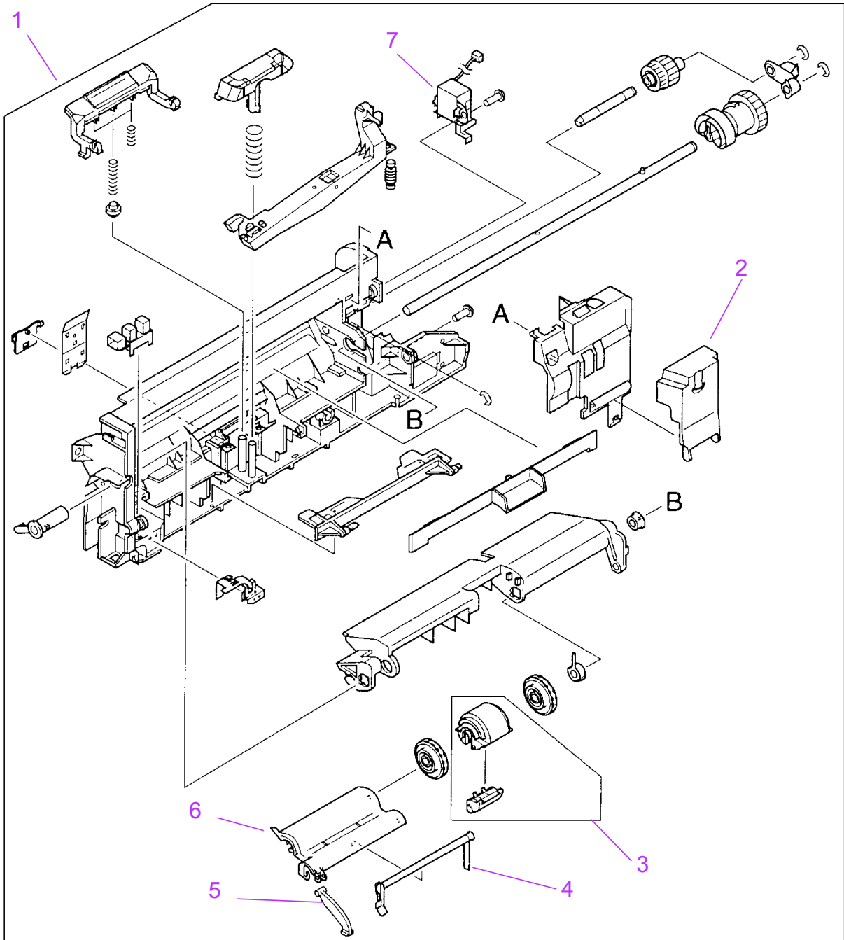
Figure 8-10 Tray 1 Pickup Assembly
