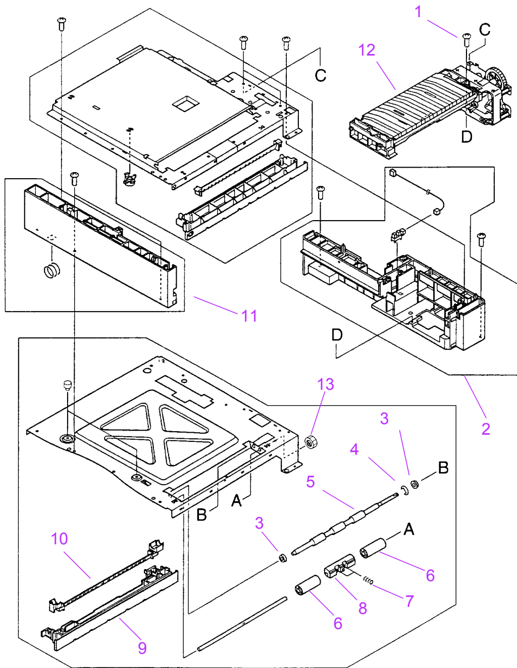
Figure 8-21 Internal Components of 250-sheet Module (1 of 2)
