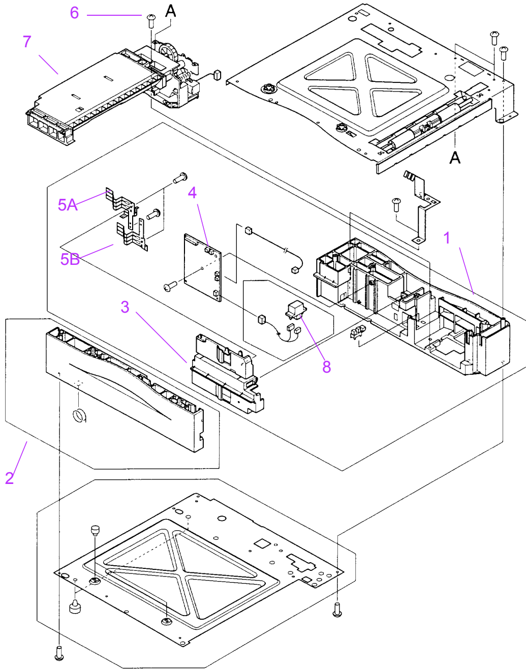
Figure 8-22 Internal Components of 250-sheet Feeder (2 of 2)
