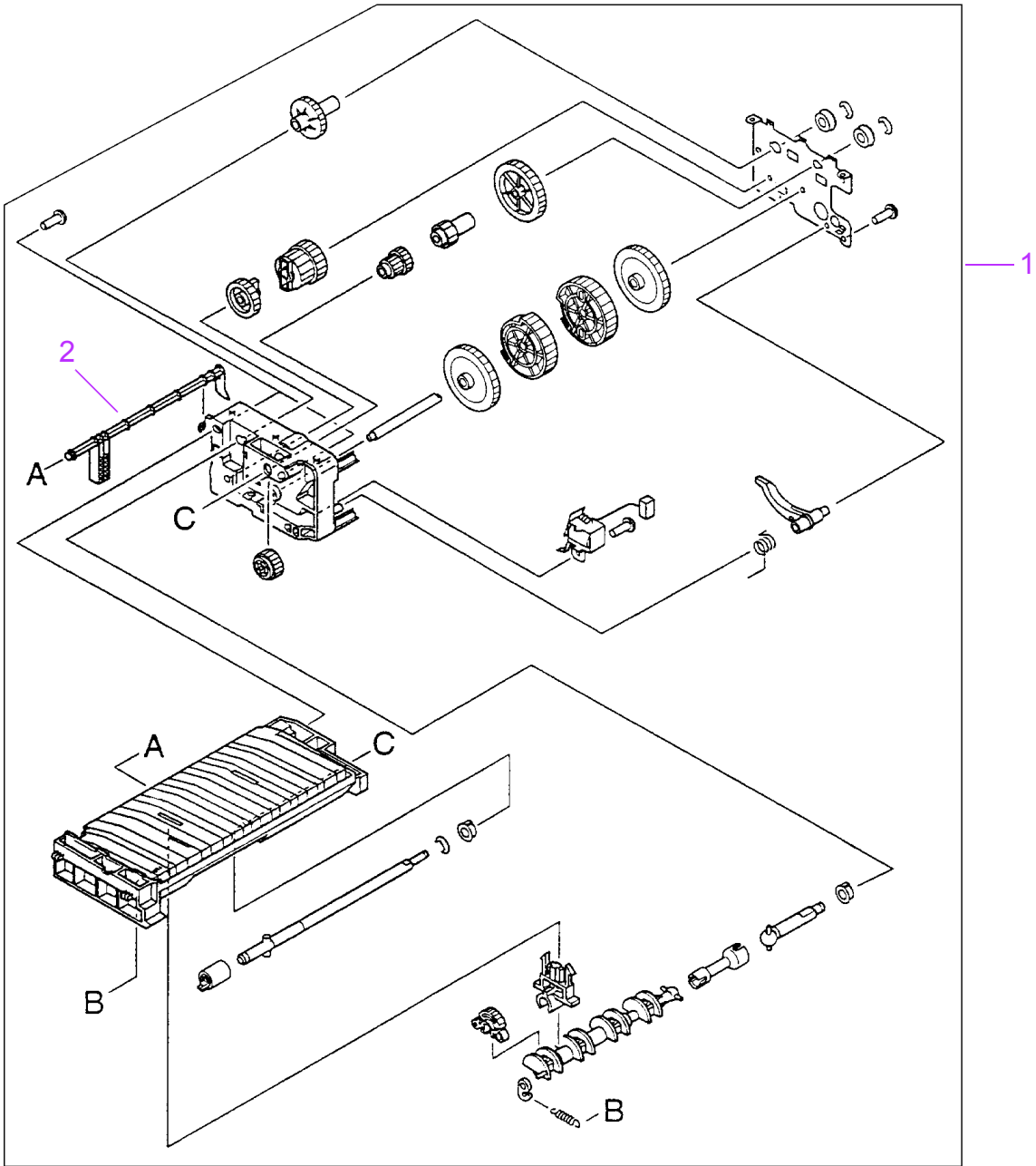
Figure 8-23 Upper Paper Pickup Drive Assembly
