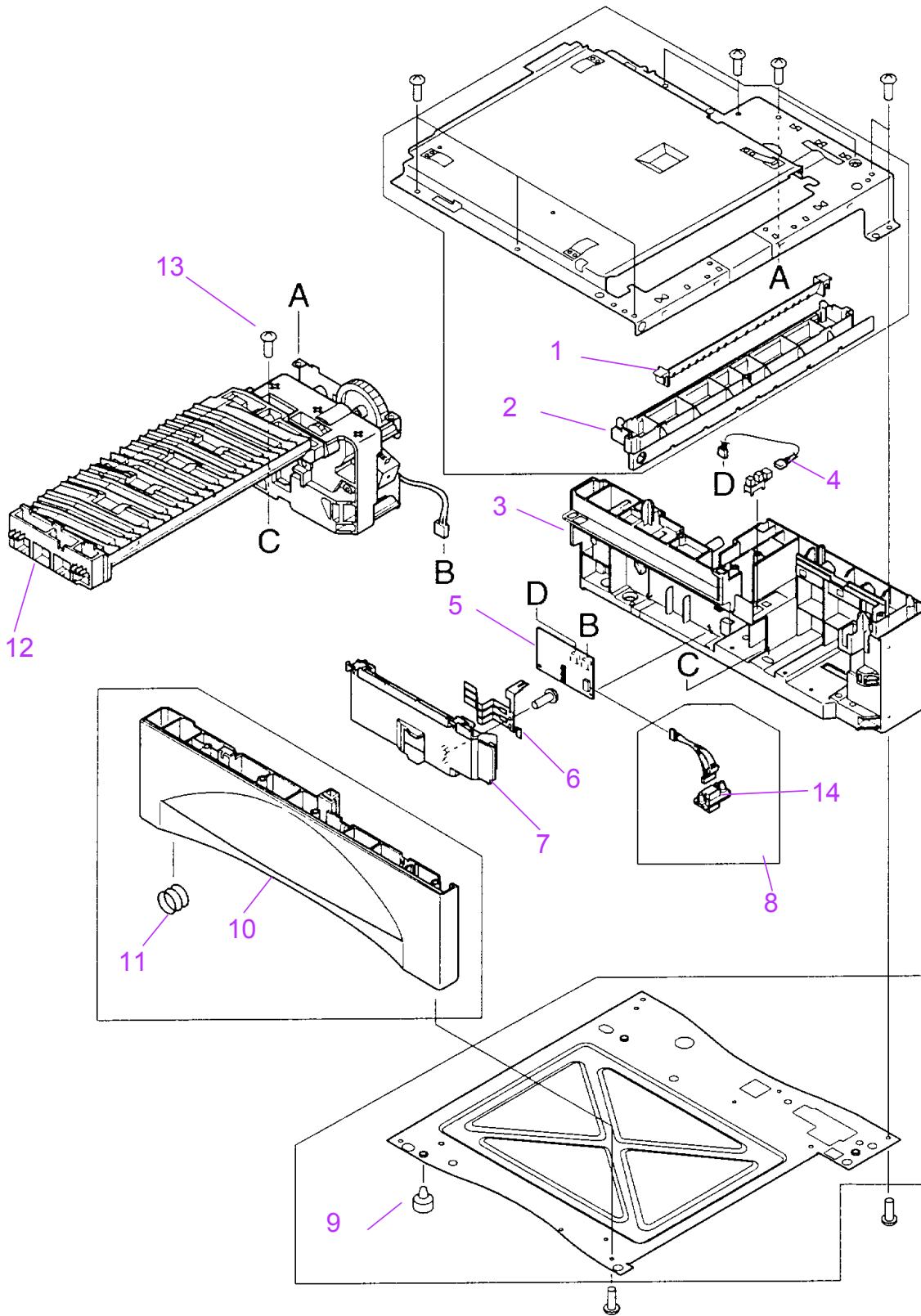
Figure 8-18 Internal Components of 500-Sheet Feeder
