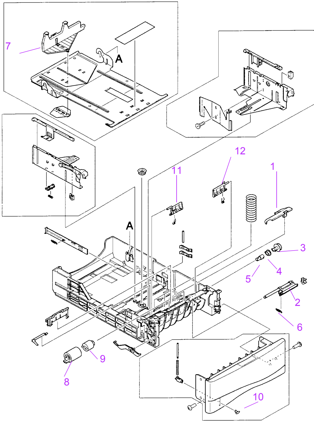
Figure 8-20 500-sheet Tray
