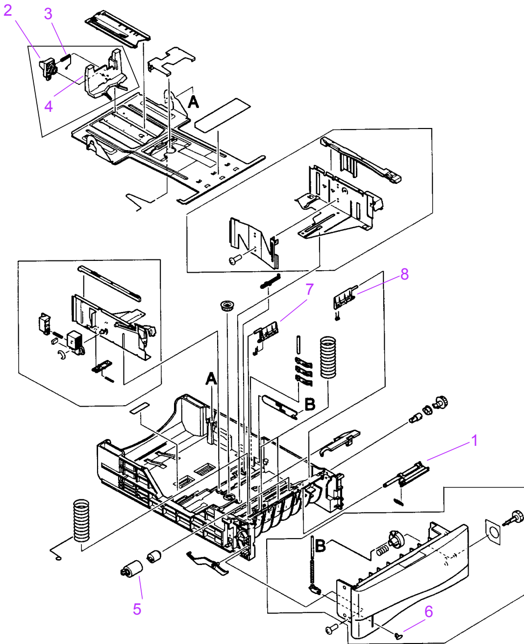
Figure 8-27 Optional 500-sheet Universal Tray Assembly
