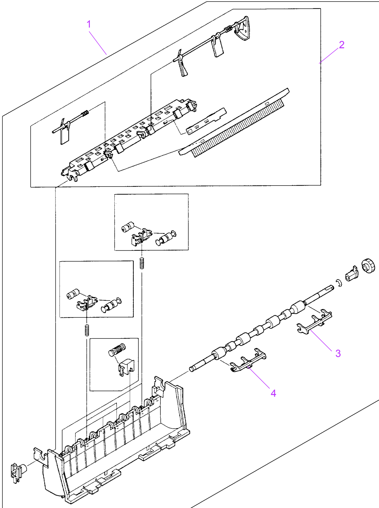
Figure 8-15 Delivery Assembly
