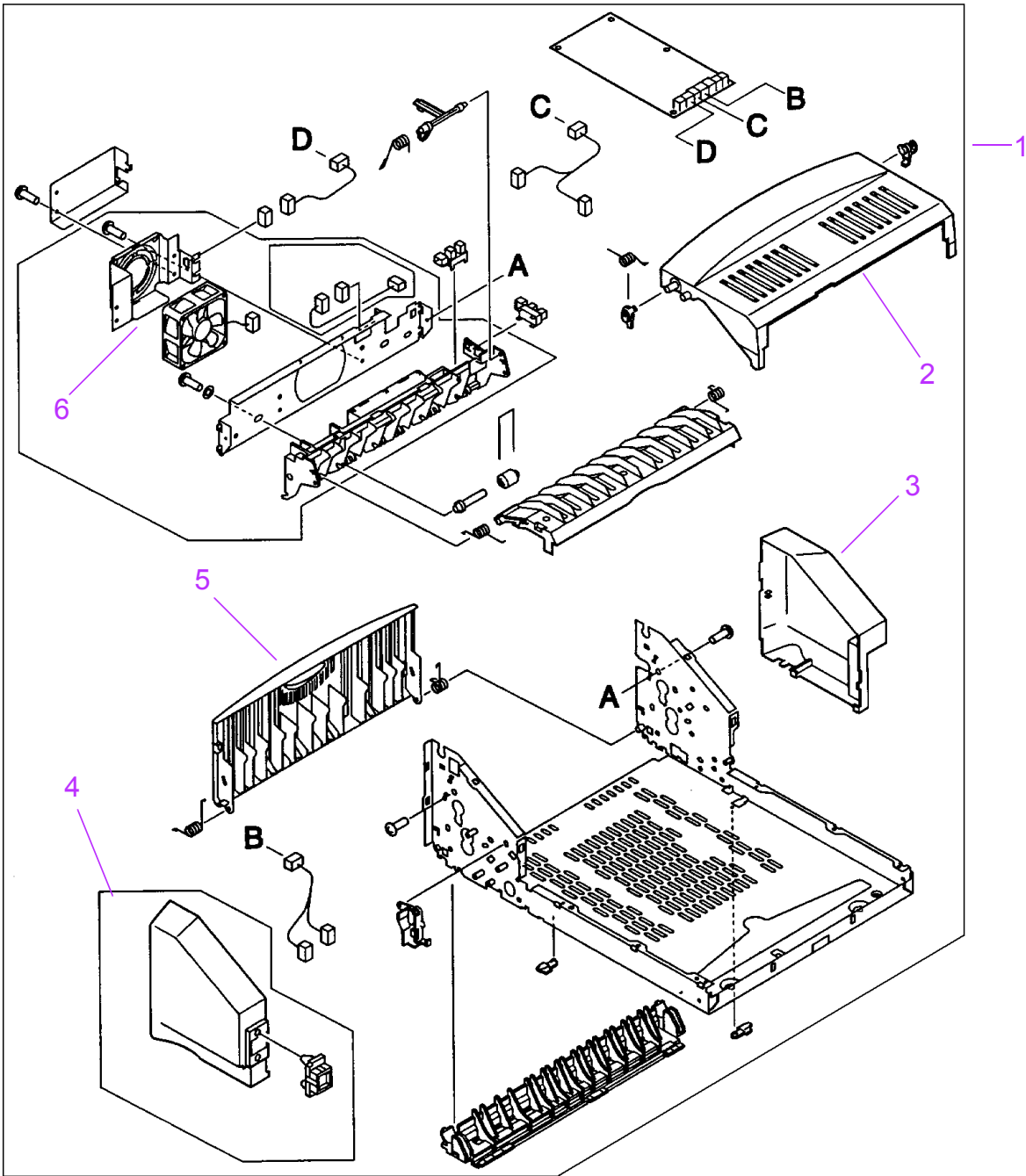
Figure 8-29 Internal Components of Duplexer
