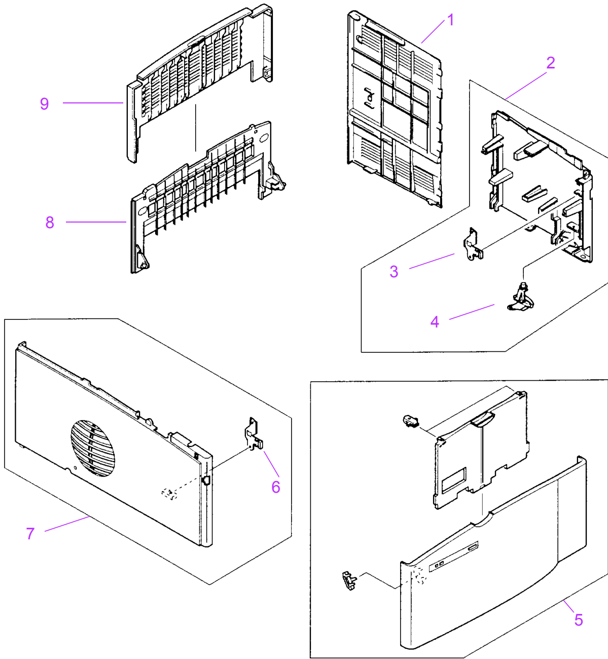
Figure 8-2 External Covers and Panels
