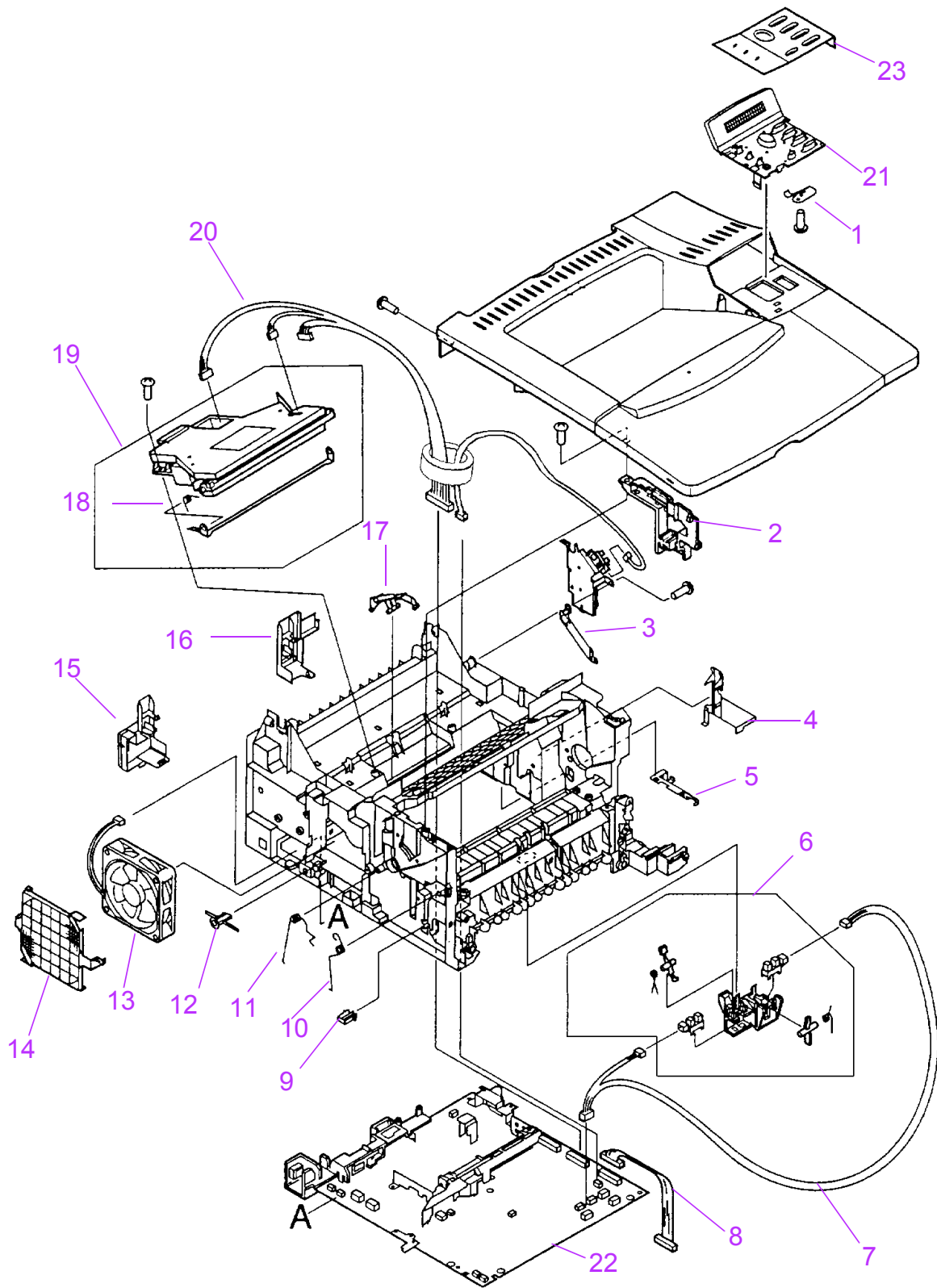
Figure 8-5 Internal Components (2 of 3)
