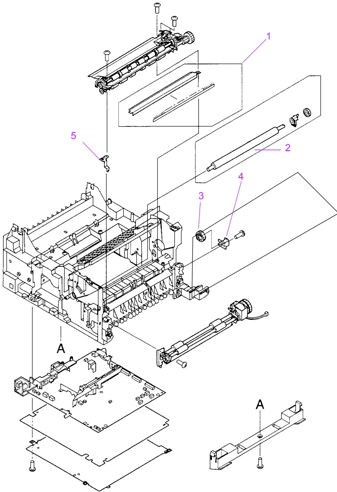
Figure 8-6 Internal Components (3 of 3)
