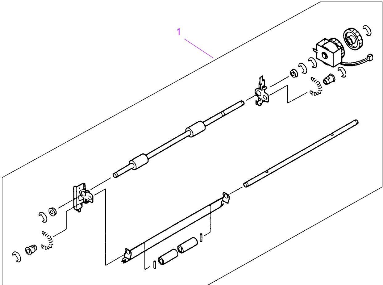
Figure 8-12 Paper Feed Assembly
