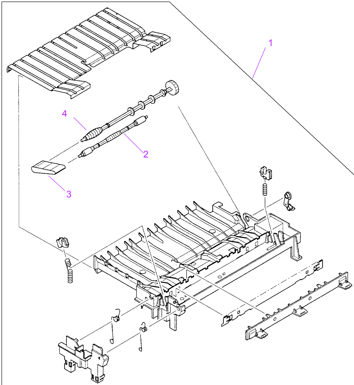
Figure 8-14 Paper Feed Guide Assembly
